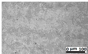
Microstructure after ageing
